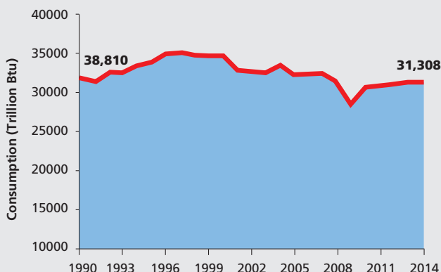
Graph 6.3: Per capita energy consumption
