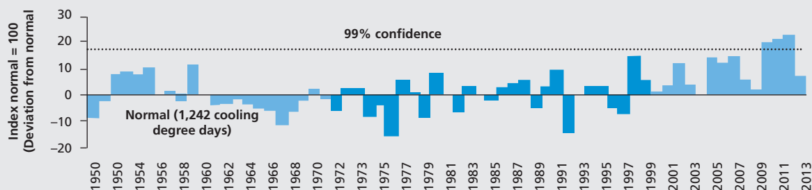
Graph 5.3: Annual deviations from normal cooling degree days (1950-2013)
