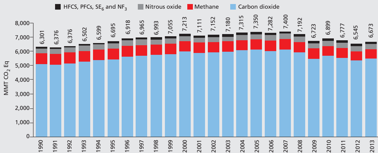
Graph 1.3: Greenhouse gas emissions, by gas, 1990-2013
